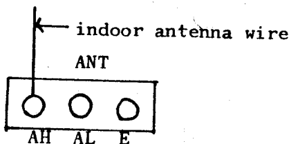
Short Indoor Antenna (Length: Abt 2M)
